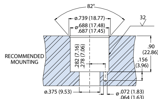
RECOMMENDED MOUNTING
