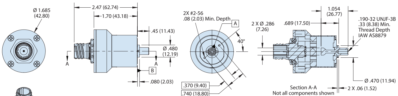
D Connector option D38999/24
